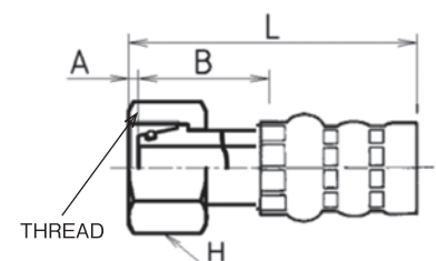
24° CONE FEMALE
