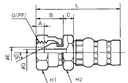
female parallel pipe G thread type (male 30° seat)
